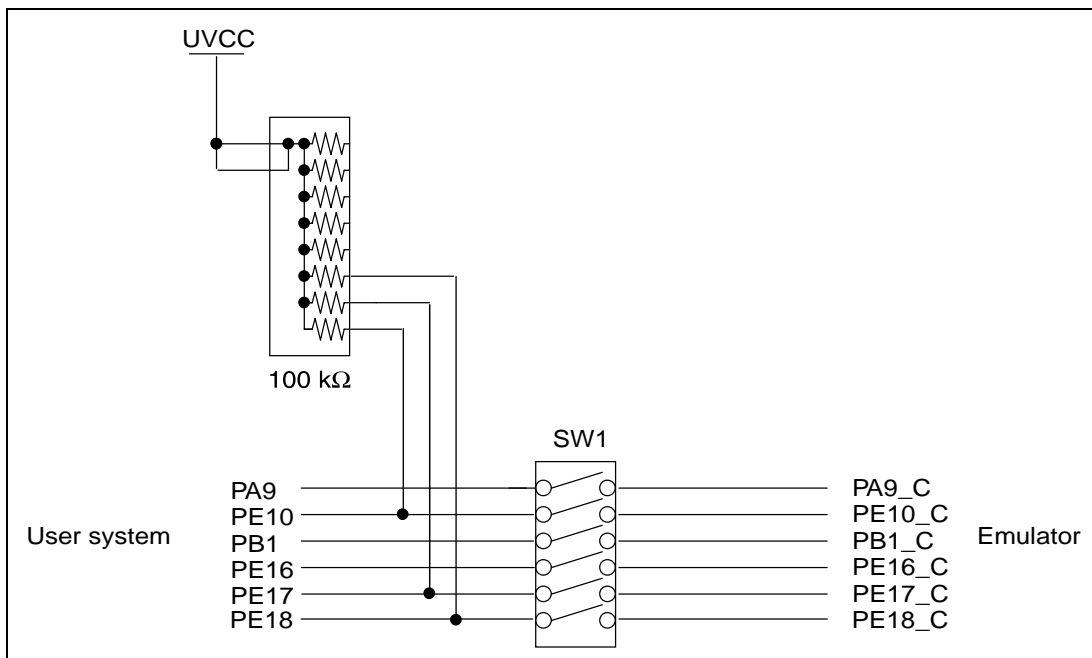
Figure 3 Circuit for Masking Signals
